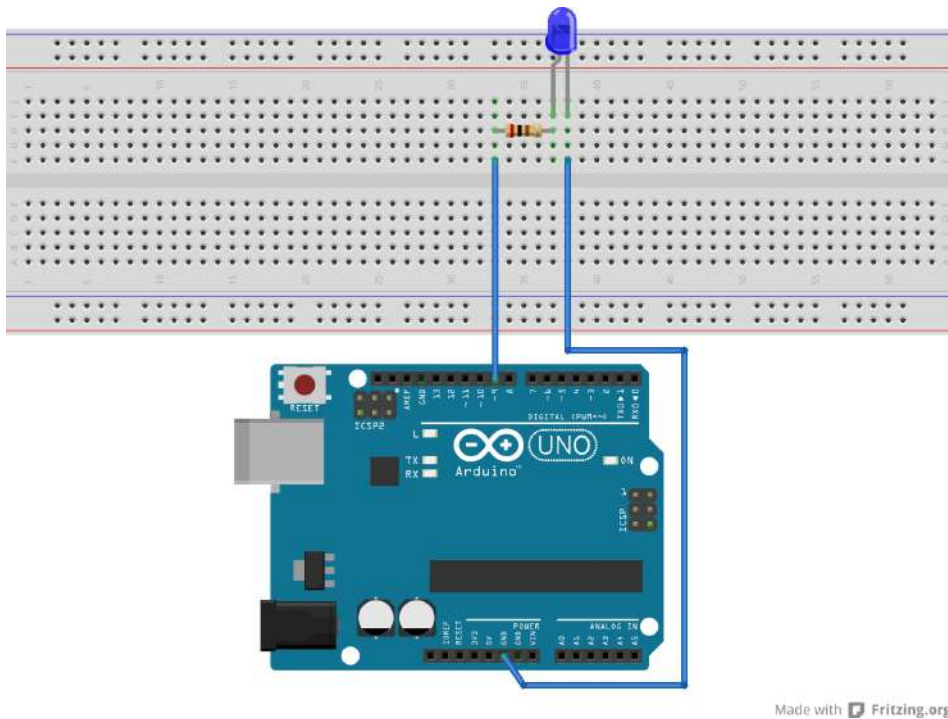
Figure 3-8: LED output (Image made with Fritzing)
