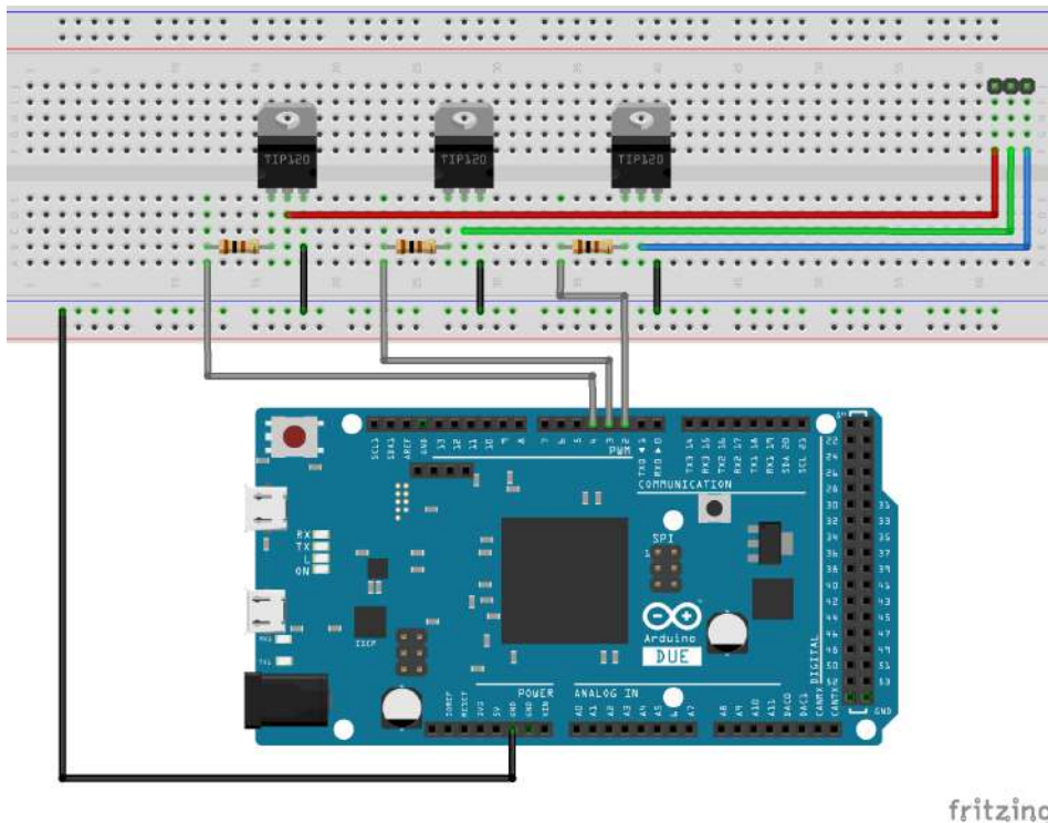
Figure 19-4: Schematic (Image created with Fritzing)
