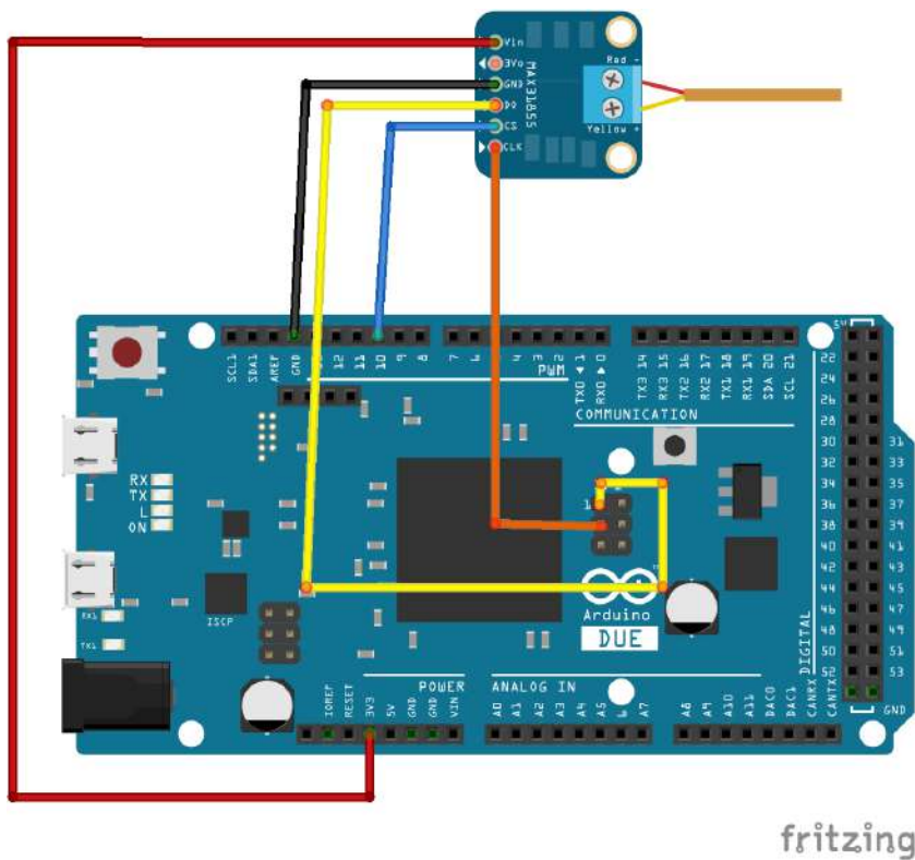
Figure 7-3: Hardware layout image created with Fritzing
