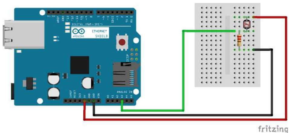
Figure 12-6: Project schematic (Image created with Fritzging)
