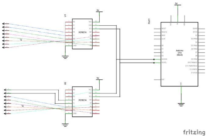
Figure 25-6: Beginning schematic work (Image created with Fritzing)
